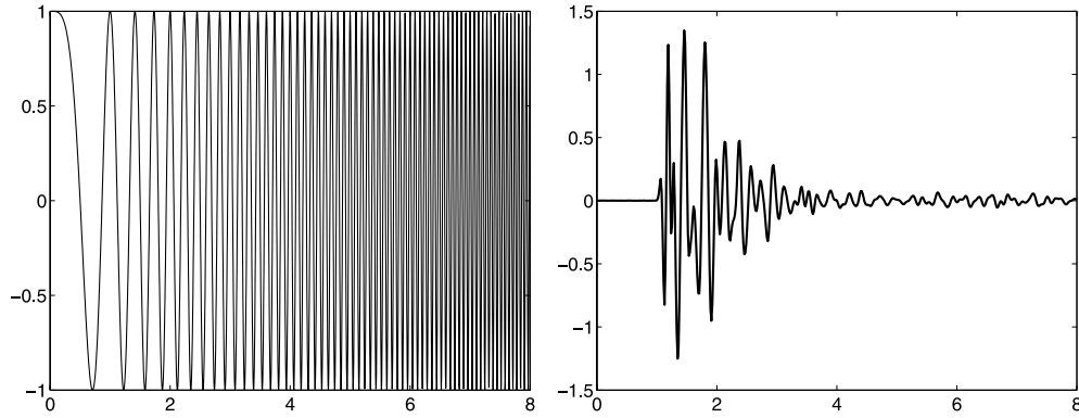
Figure 3. Chirp signal f = \cos(2\pi x^2) (left). Seismic signal (right).
